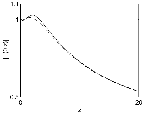
FIG. 4. Grid convergence for \epsilon = 0.04 , z_{\max} = 20 , r_{\max}/z_{\max} = 1 , h_z = \lambda_z/10 , for h_r = \lambda_z/2 (solid line), h_r = \lambda_z/4 (dotted line), and h_r = \lambda_z/8 (dashed line).
